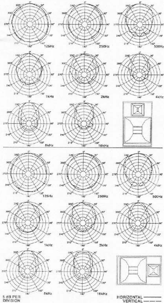
FIGURE 3 — MTH-2.5/64B Polar Response
